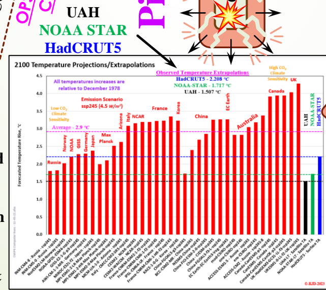
CSS-30 - CMIP6 Computer Models
