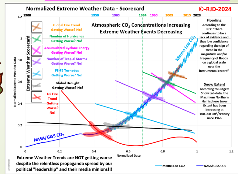
CSS-52 - Extreme Weather Events
