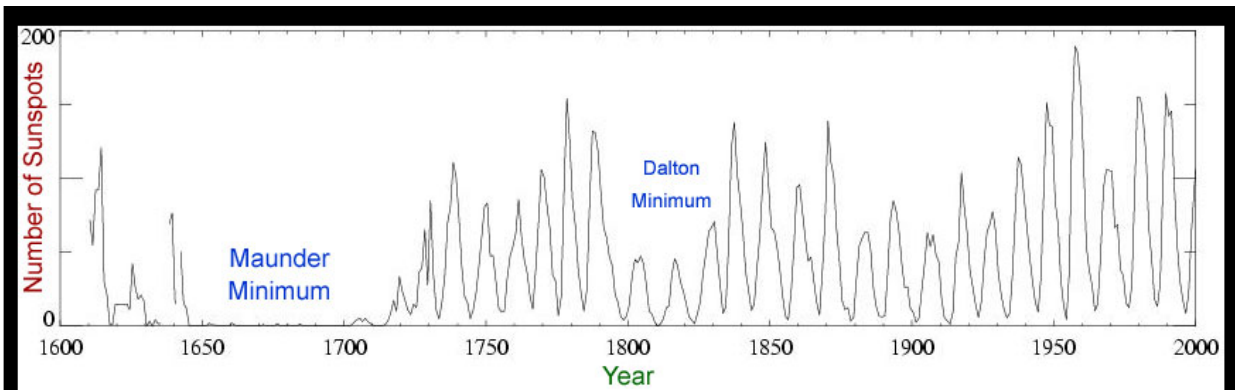
This graph shows the number of sunspots seen each year for 400 years (from 1600 to 2000). There were almost no sunspots during the Maunder Minimum. During the Dalton Minimum, there were fewer sunspots than normal. Image courtesy NASA (modified by Windows to the Universe staff).
