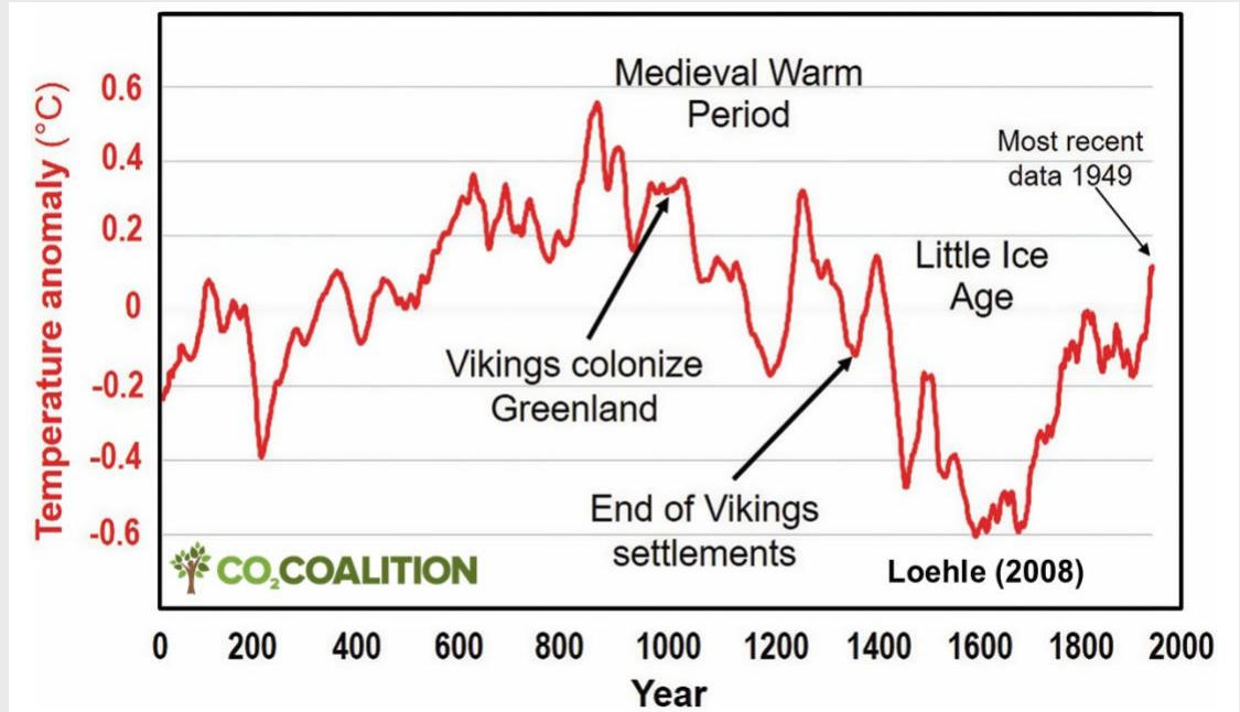
Figure19: The Medieval Warm Period and the Little Ice Age 33
