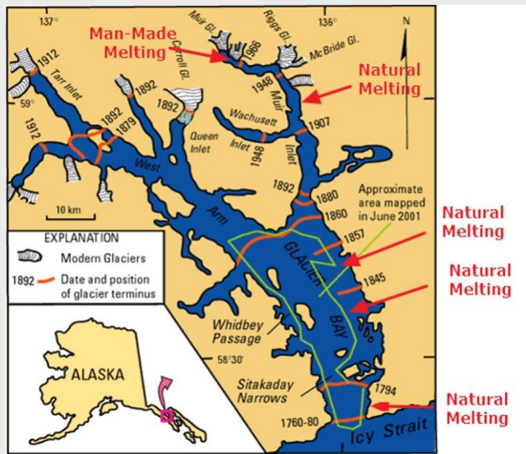
Figure 20: Glacier Bay Alaska showing the retreat of the glaciers (Source: CO 2 Coalition) 34
